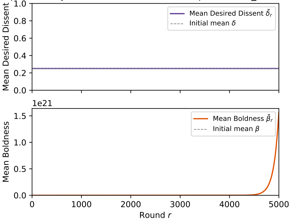
Population Dynamics (k=1, C=0.0000, bp=1%, self_censor-
