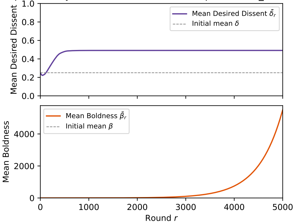
Population Dynamics ( k=1 , C=0.0020 , bp=0\% , self\_censor=0 )
