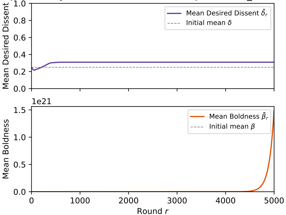
Population Dynamics (k=1, C=0.0020, bp=1%, self_censor-
