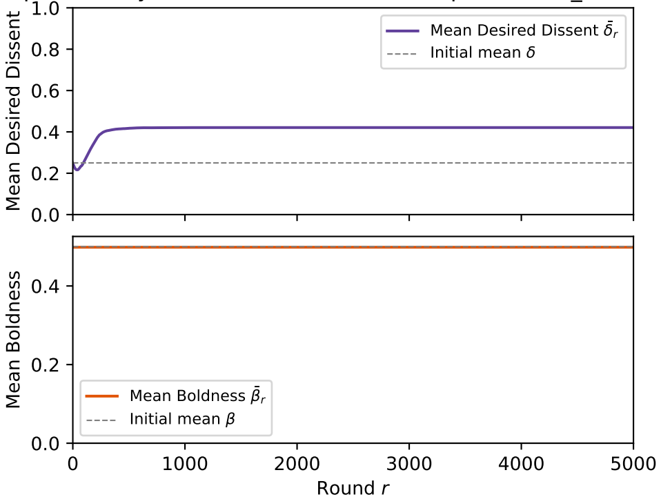
Population Dynamics ( k=1 , C=0.0030 , bp=0\% , self_censor-
