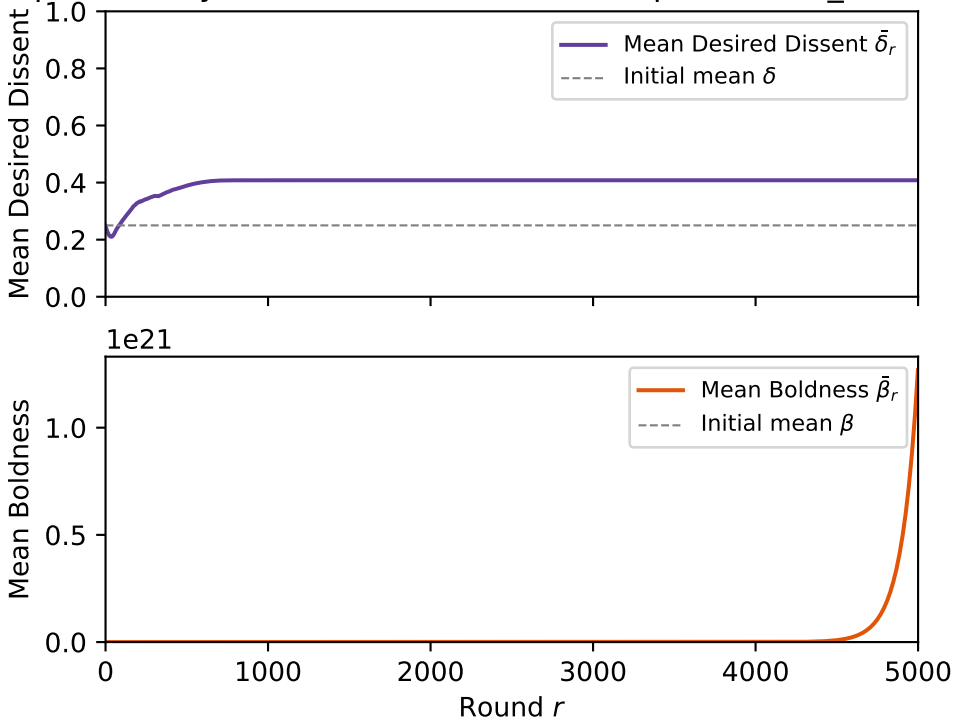
Population Dynamics (k=1, C=0.0040, bp=1%, self_censor-
