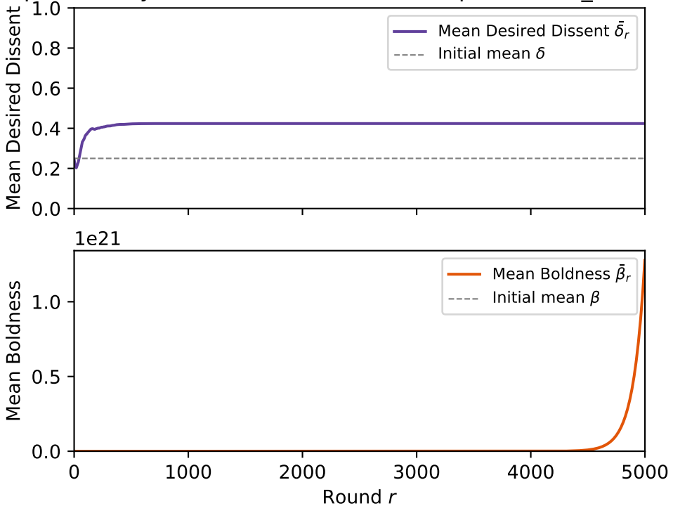
Population Dynamics (k=1, C=0.0090, bp=1%, self_censor-
