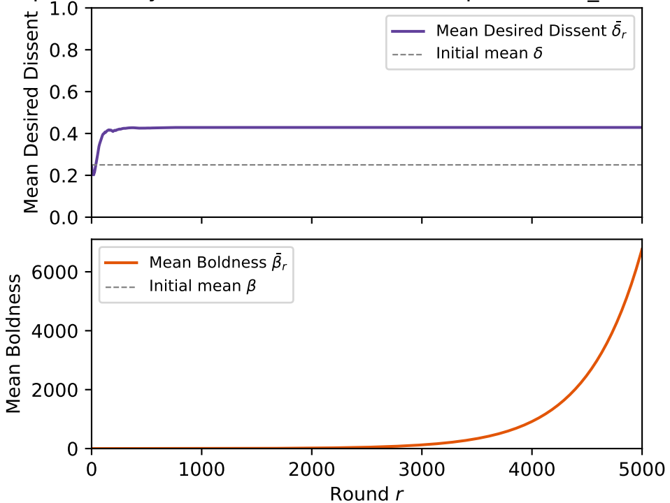
Population Dynamics ( k=1 , C=0.0100 , bp=0\% , self\_censor=0 )
