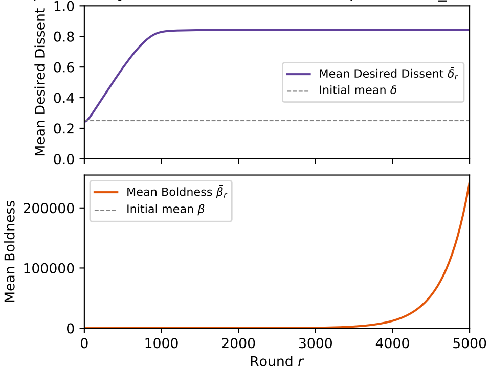
Population Dynamics ( k=3 , C=0.0010 , bp=0\% , self\_censor=0\% )
