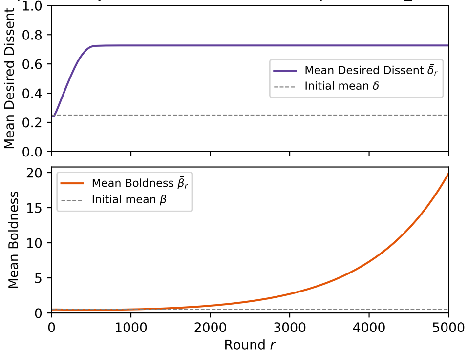
Population Dynamics ( k=3 , C=0.0020 , bp=0\% , self\_censor=
