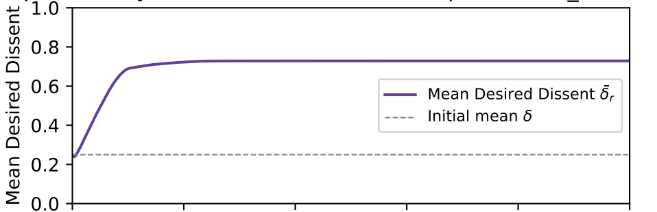
Population Dynamics (k=3, C=0.0020, bp=1%, self_censor-
