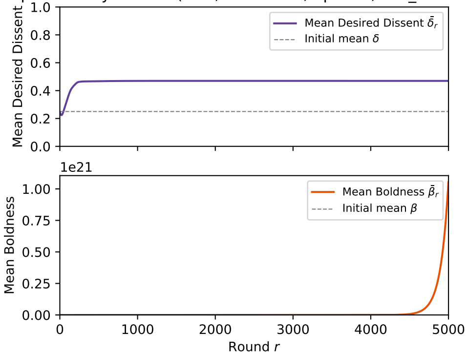
Population Dynamics ( k=3 , C=0.0050 , bp=1\% , self_censor)
