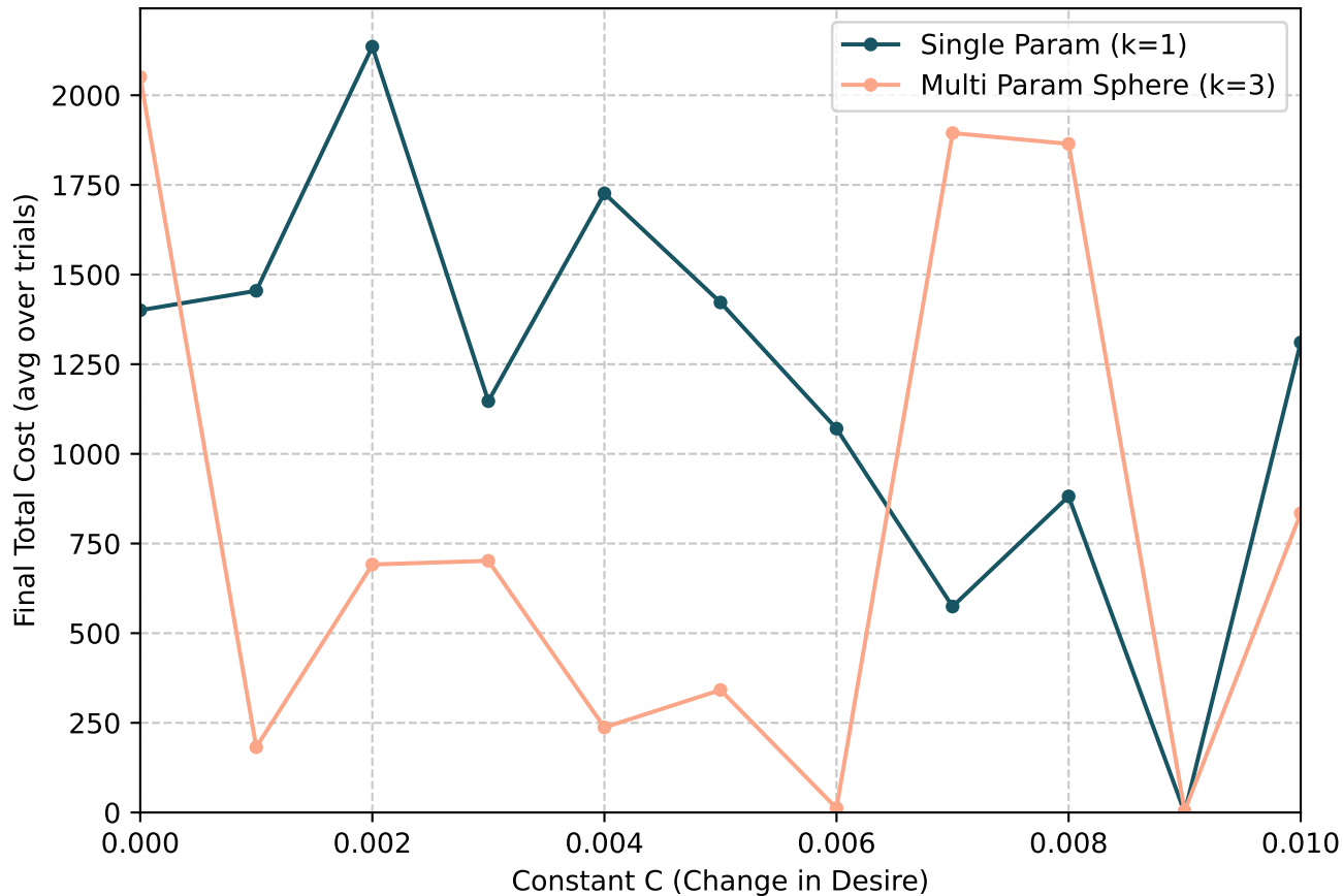
Single vs Multi Param RMHC (Sphere): C vs Final Cost
