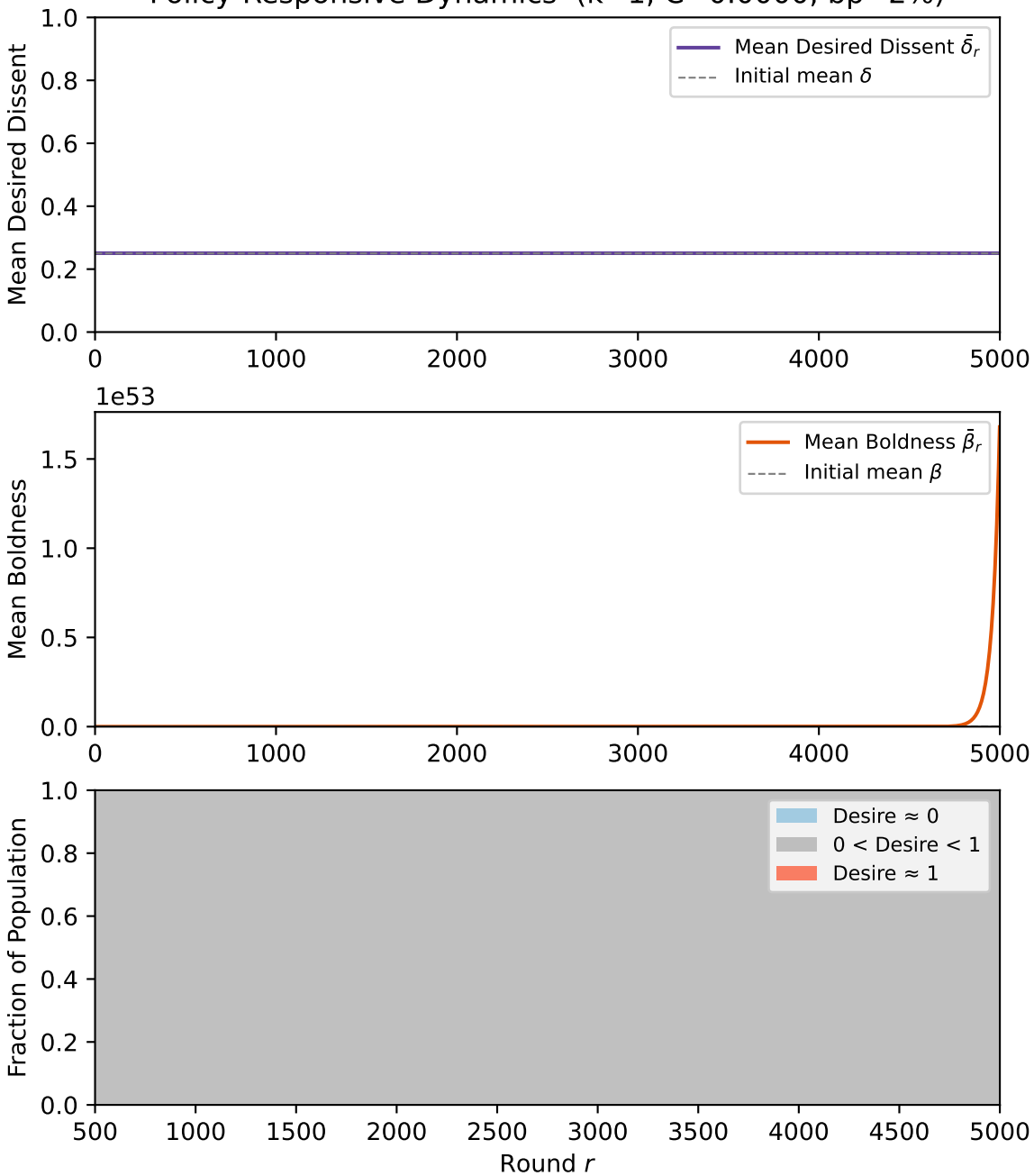
Policy-Responsive Dynamics (k=1, C=0.0000, bp=2%)
