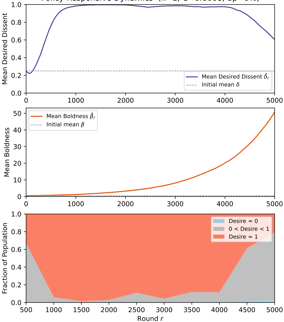
Policy-Responsive Dynamics ( k=1 , C=0.0008 , bp=0\% )
