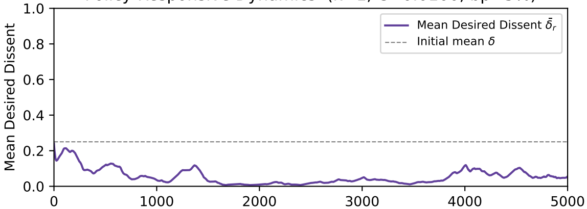
Policy-Responsive Dynamics ( k=1 , C=0.0100 , bp=5\% )
