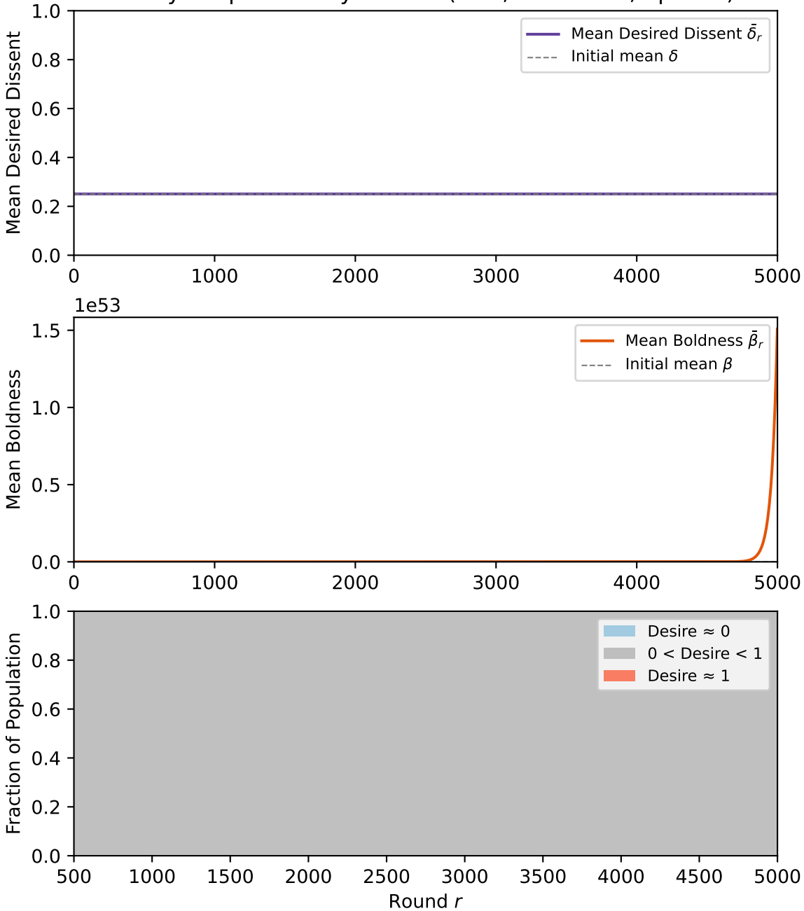
Policy-Responsive Dynamics ( k=3 , C=0.0000 , bp=2\% )
