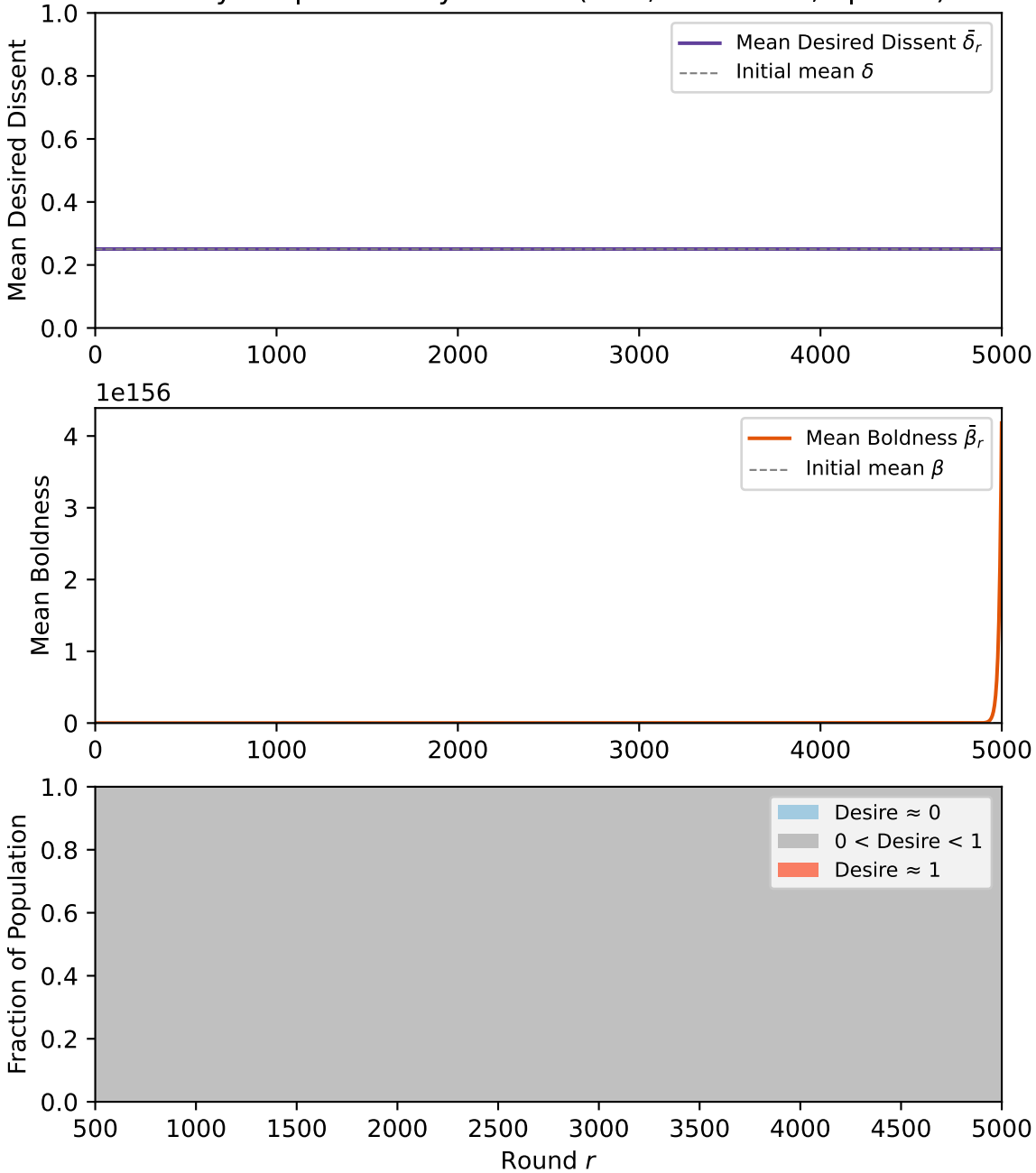
Policy-Responsive Dynamics ( k=3 , C=0.0000 , bp=8\% )
