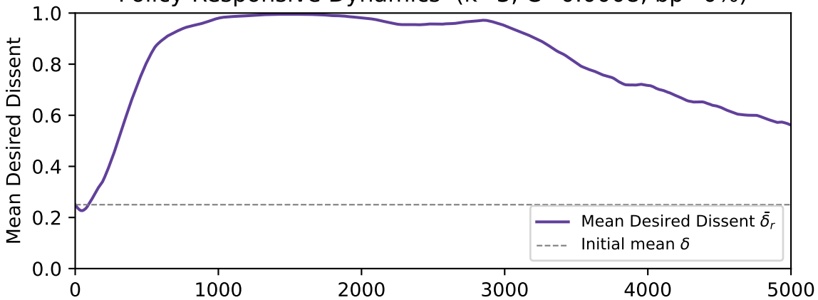
Policy-Responsive Dynamics ( k=3 , C=0.0008 , bp=0\% )
