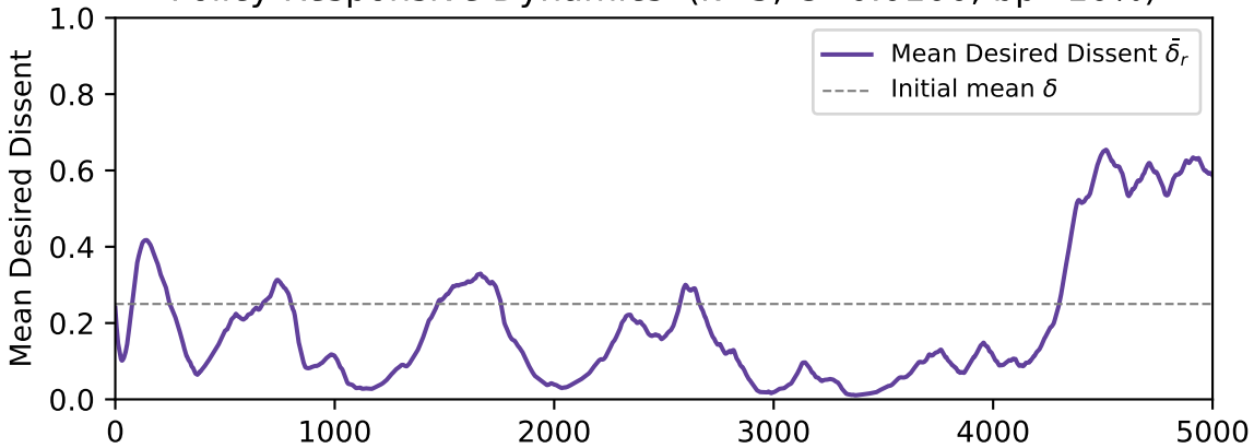
Policy-Responsive Dynamics ( k=3 , C=0.0100 , bp=10\% )
