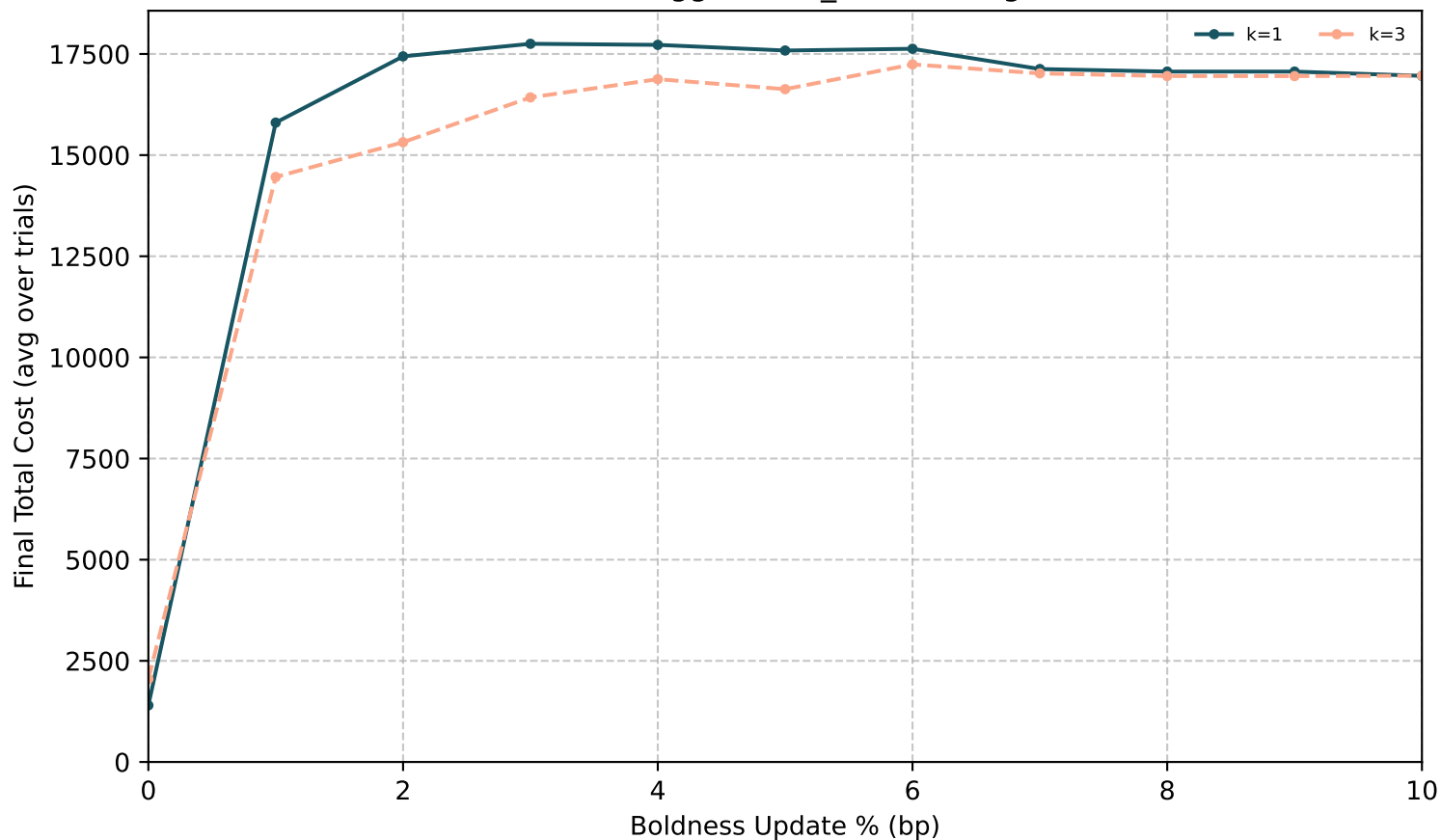
RMHC: Final Cost [trigger=self_censor, target=boldness]
