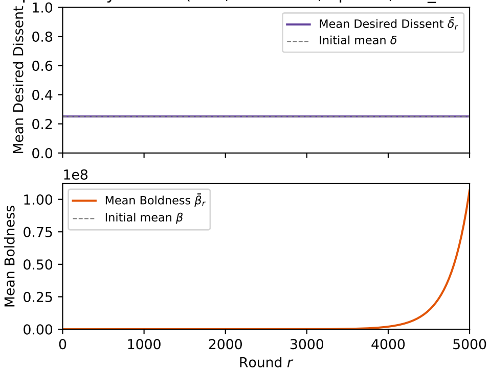
Population Dynamics ( k=1 , C=0.0000 , bp=0\% , self\_censor )
