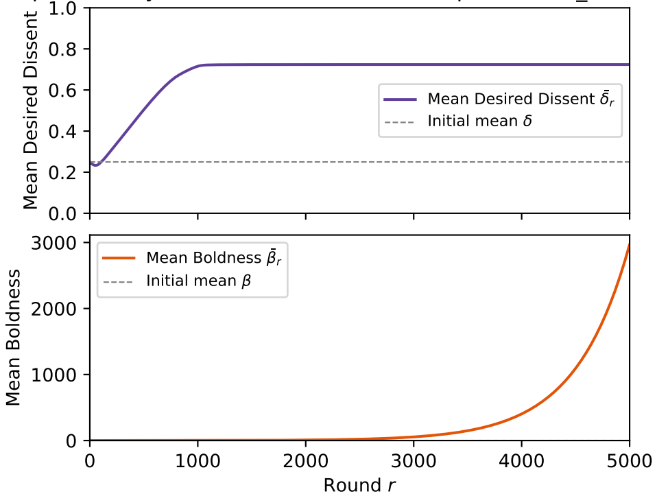
Population Dynamics ( k=1 , C=0.0010 , bp=0\% , self\_censor=0 )
