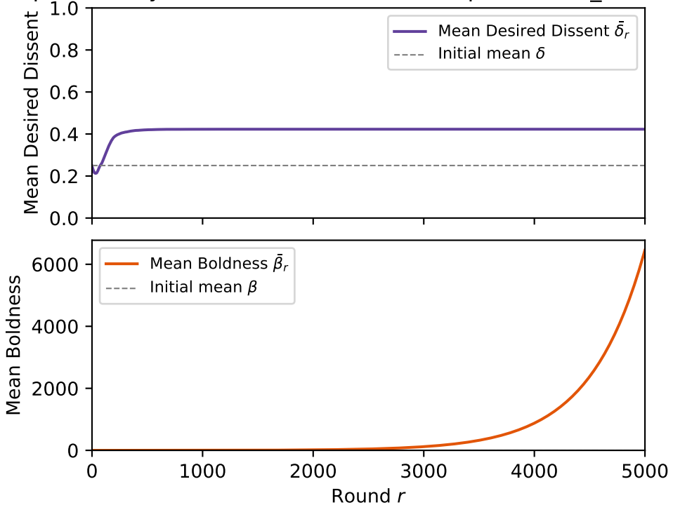
Population Dynamics ( k=1 , C=0.0040 , bp=0\% , self\_censor=0 )
