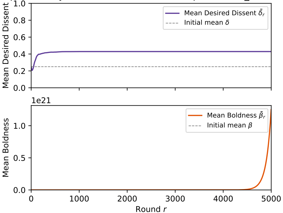
Population Dynamics ( k=1 , C=0.0070 , bp=1\% , self_censor-
