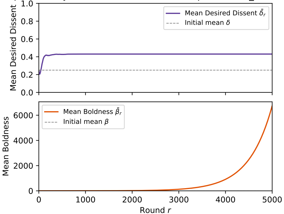
Population Dynamics ( k=1 , C=0.0080 , bp=0\% , self\_censor )
