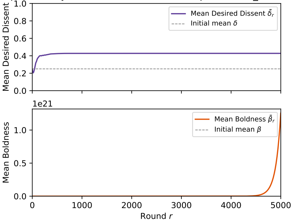
Population Dynamics ( k=1 , C=0.0080 , bp=1\% , self_censor-
