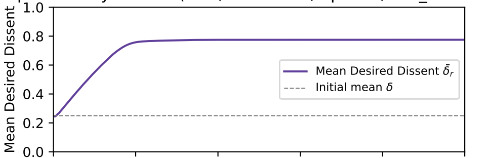
Population Dynamics ( k=3 , C=0.0010 , bp=1\% , self_censor-
