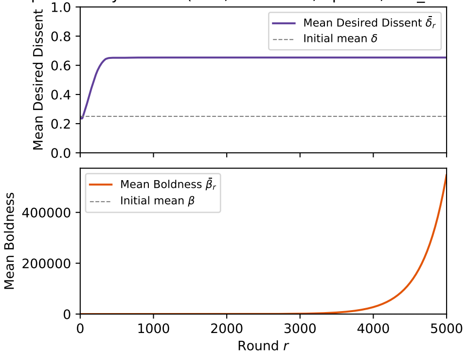
Population Dynamics ( k=3 , C=0.0030 , bp=0\% , self\_censor )
