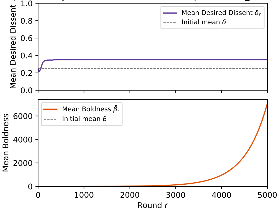
Population Dynamics ( k=3 , C=0.0060 , bp=0\% , self\_censor=0 )
