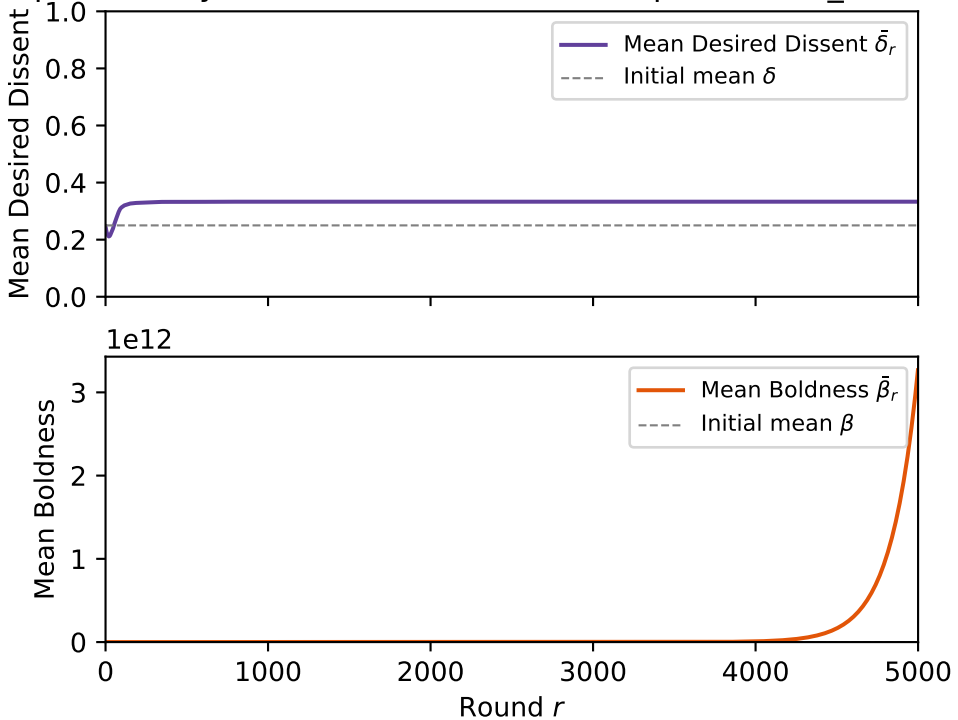
Population Dynamics ( k=3 , C=0.0070 , bp=1\% , self_censor-
