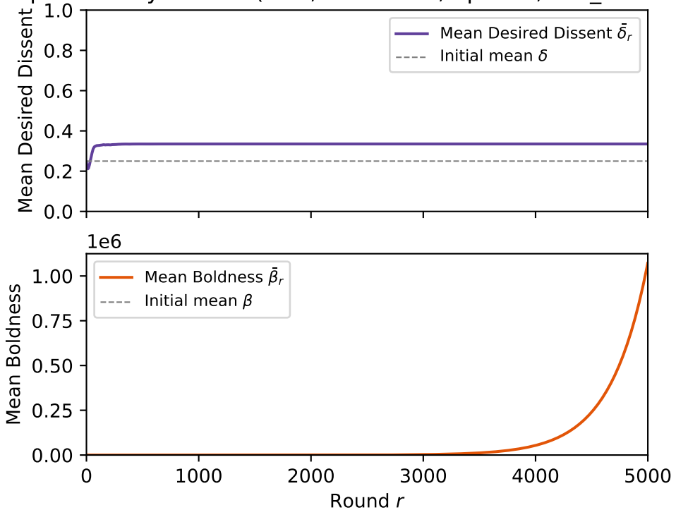
Population Dynamics ( k=3 , C=0.0100 , bp=0\% , self\_censor )
