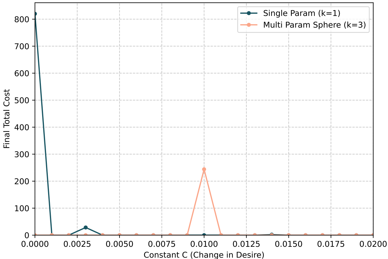
Single vs Multi Param RMHC (Sphere): C vs Cost
