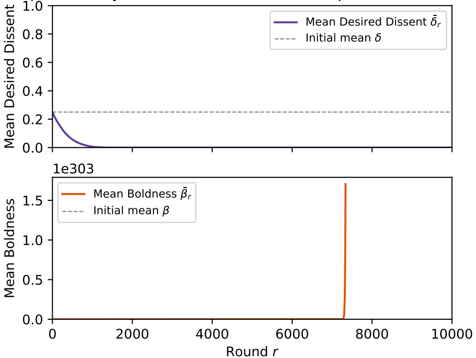
Population Dynamics ( k=1 , C=0.0010 , bp=10\% , mixed \rightarrow a
