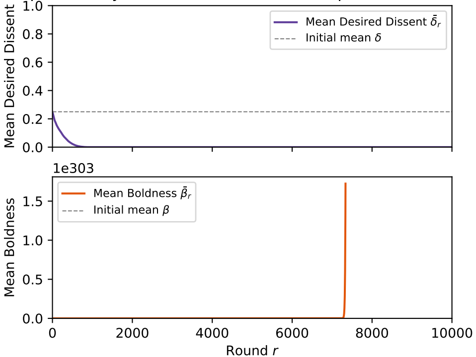
Population Dynamics ( k=1 , C=0.0020 , bp=10\% , mixed \rightarrow a
