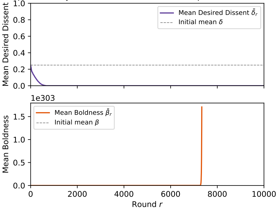
Population Dynamics ( k=1 , C=0.0030 , bp=10\% , mixed \rightarrow a
