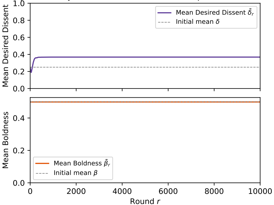
Population Dynamics (k=1, C=0.0050, bp=0%, mixed→all)
