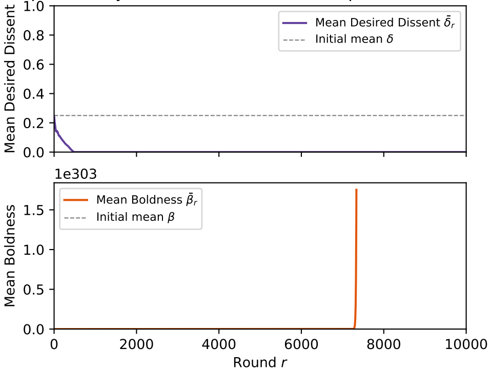
Population Dynamics ( k=1 , C=0.0070 , bp=10\% , mixed \rightarrow a
