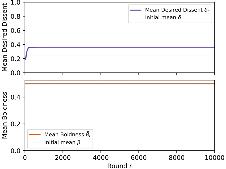
Population Dynamics (k=1, C=0.0080, bp=0%, mixed→all)
