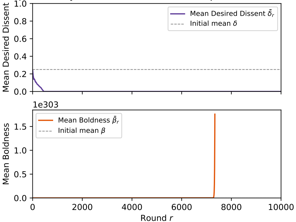
Population Dynamics ( k=1 , C=0.0080 , bp=10\% , mixed \rightarrow a
