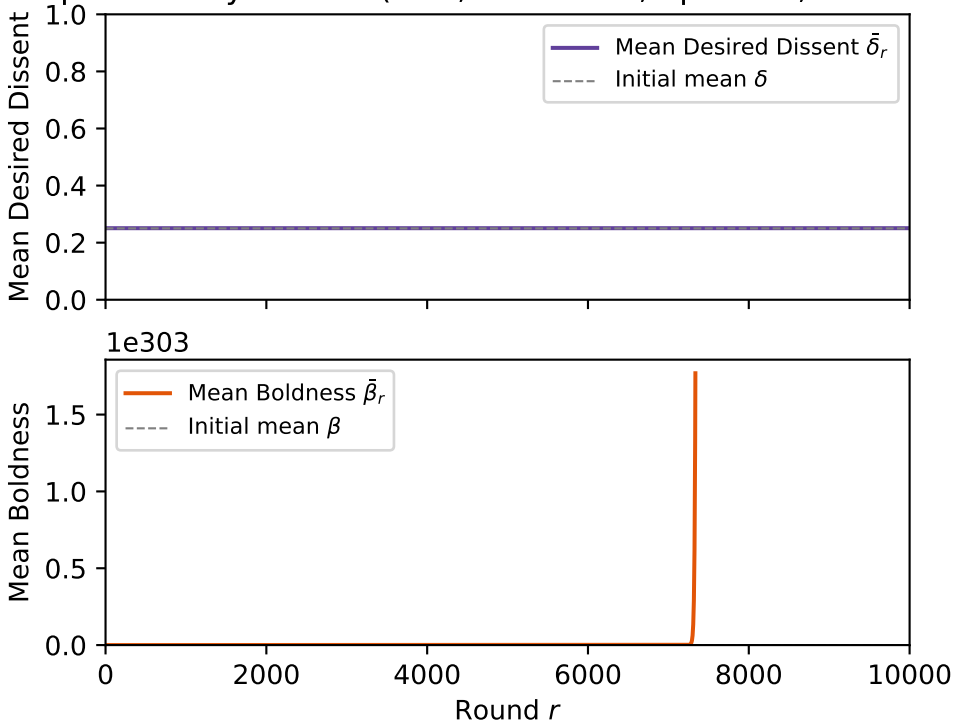
Population Dynamics ( k=3 , C=0.0000 , bp=10\% , mixed \rightarrow a )
