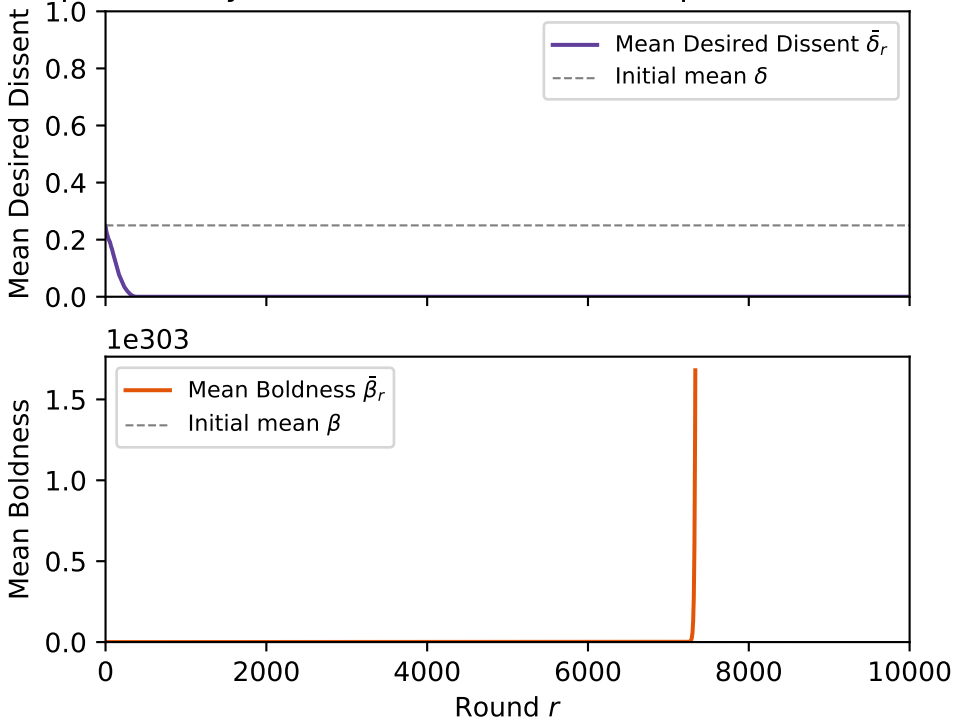
Population Dynamics ( k=3 , C=0.0050 , bp=10\% , mixed \rightarrow a
