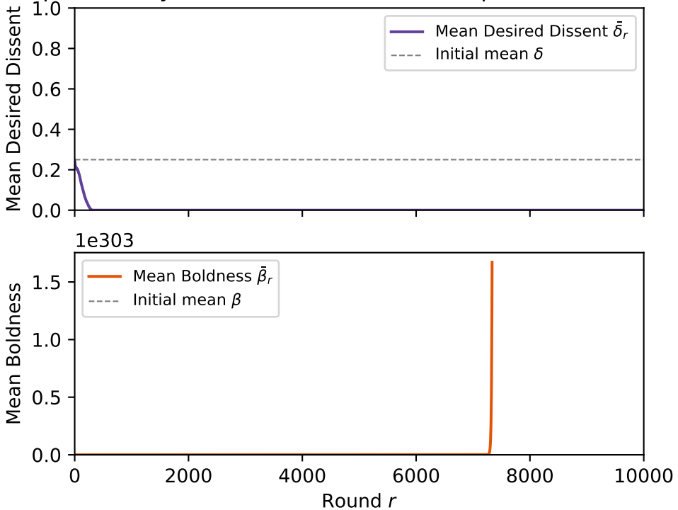
Population Dynamics (k=3, C=0.0070, bp=10%, mixed→a
