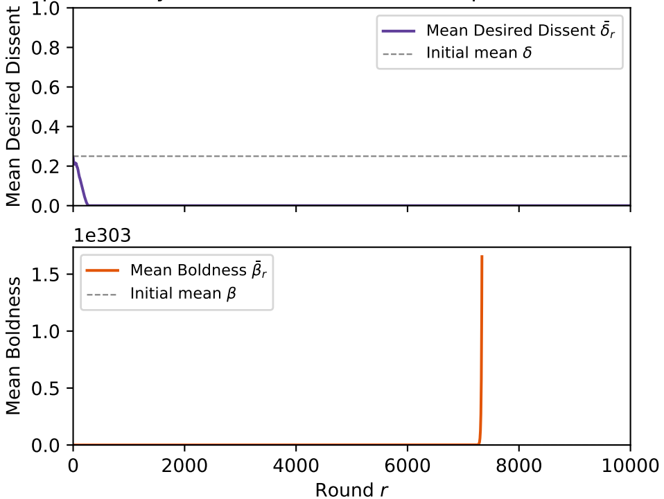
Population Dynamics (k=3, C=0.0090, bp=10%, mixed→a
