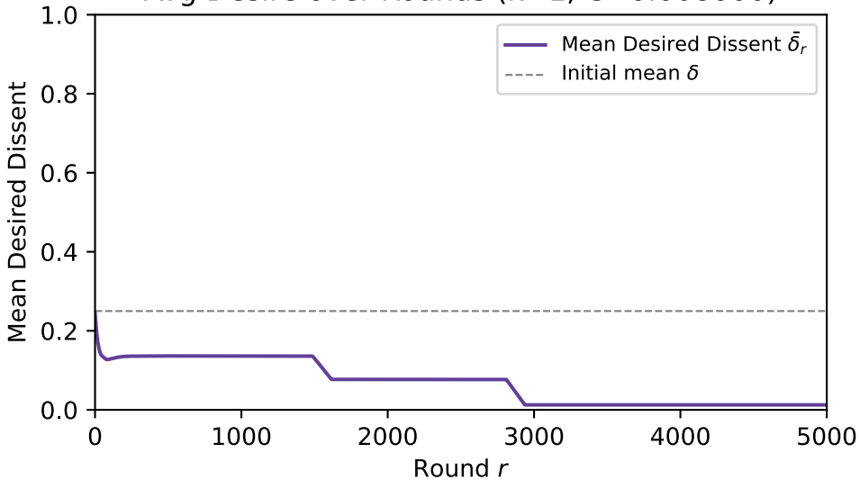
Avg Desire over Rounds ( k=1 , C=0.008000 )
