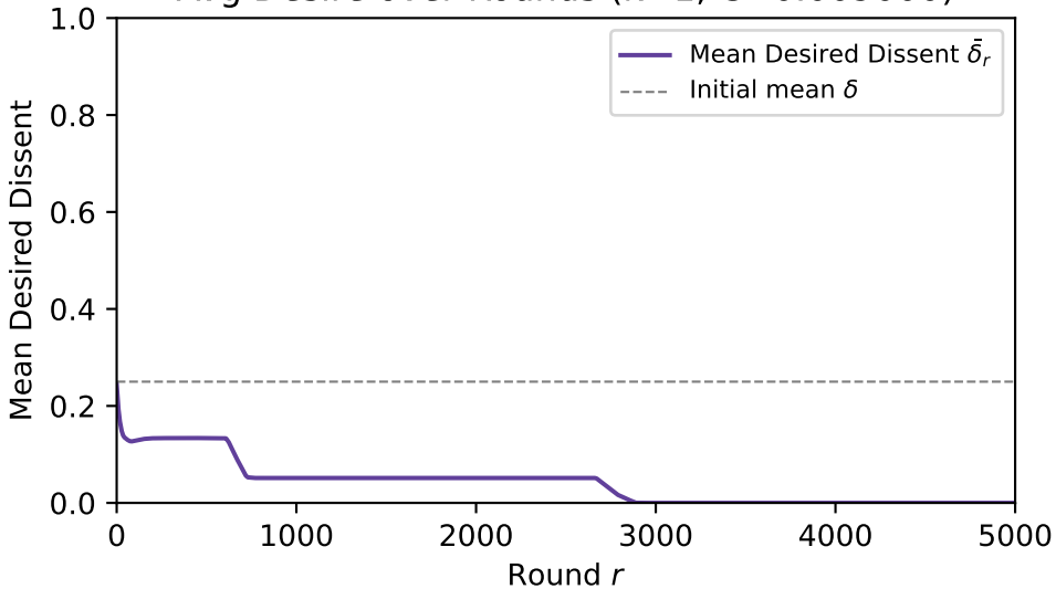
Avg Desire over Rounds (k=1, C=0.009000)
