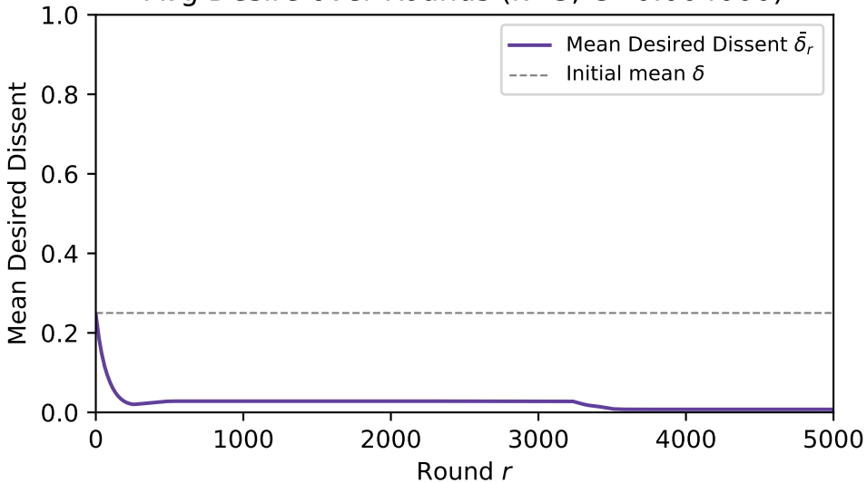
Avg Desire over Rounds (k=3, C=0.004000)
