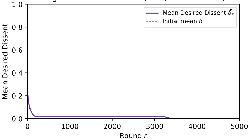
Avg Desire over Rounds ( k=3 , C=0.006000 )
