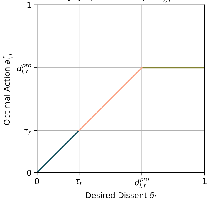
(A) \nu_r < 1 and \tau_r < d_{i,r}^{pro}
