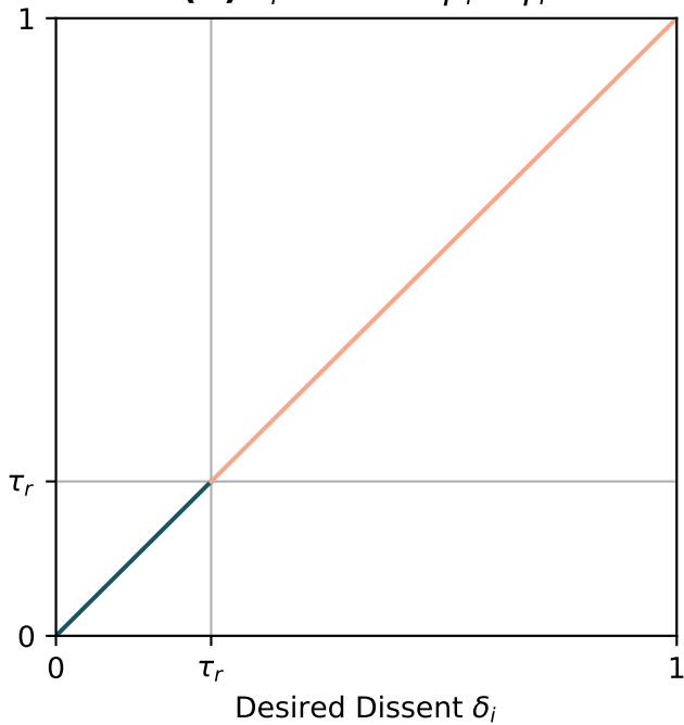
(B) \nu_r = 1 and \beta_i \geq \psi_r
