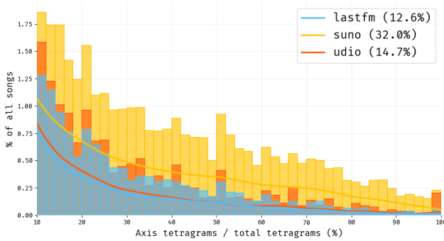
Figure 10: Distribution of the percentage of axis-based tetragrams per song across the three collections (songs with \geq 10\% axis content only). Lastfm shows 12.6%, Suno 32.0%, and Udio 14.7% of songs exceeding the 10% axis tetragram threshold.
