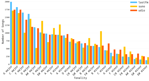
Figure 4: Distribution of most common tonalities in all three collections.
