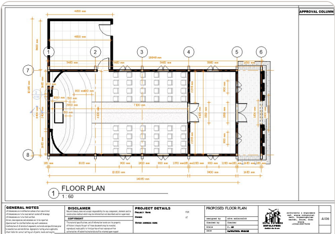
Proposed Floor Plan Documentation
