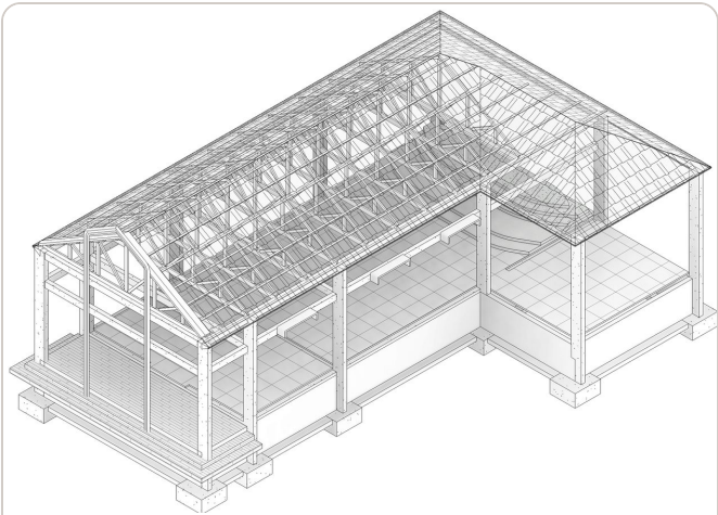
Structural BIM Model — Construction Phase
